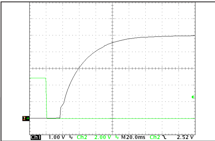
Figure 7: Turn-on transient at no load and zero output capacitance initiated by On/Off. Input voltage pre-applied. Ch 1: Vout (1 V/div). Ch 2: On/Off (2 V/div). (20 ms/div).
