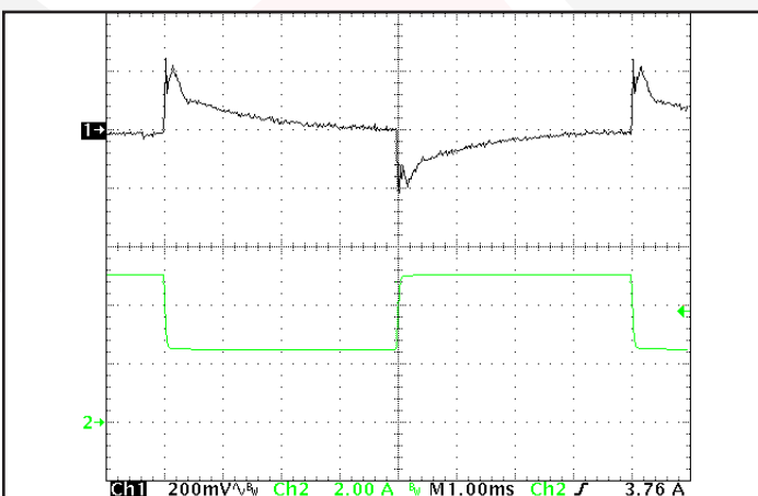
Figure 11: Output voltage response to step-change in load current 50%-100%-50% of Iout (max); dI/dt = 0.05 \text{ A}/\mu\text{s} . No external load capacitance. Ch 1: Vout (200 mV/div). Ch 2: Iout (2 A/div). (1 ms/div).
